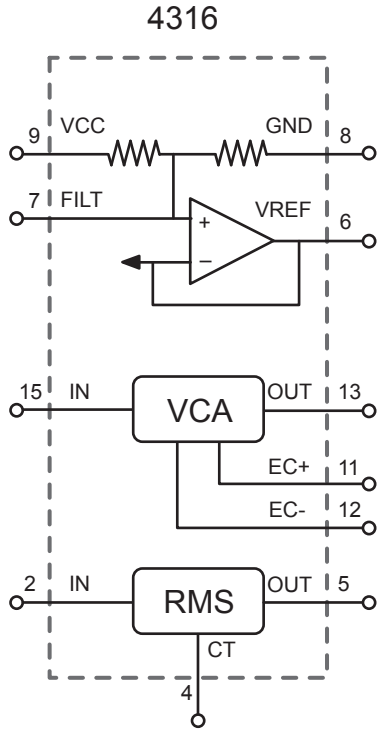
16-pin QSOP Package
