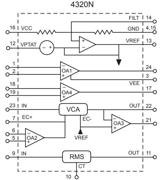
24-pin QFN package
